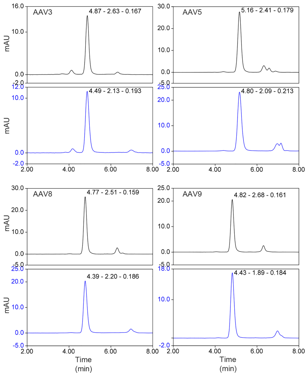
Figure 7. Chromatograms of using 3 μm SurePac Bio 550 SEC MDi column (black) and another vendor column with 2.5 μm particle size (blue) for AAV3, 5, 8, and 9 samples. Peak label: RT (min) – Resolution between monomer and HMWS – PWHH (peak width at half height).
