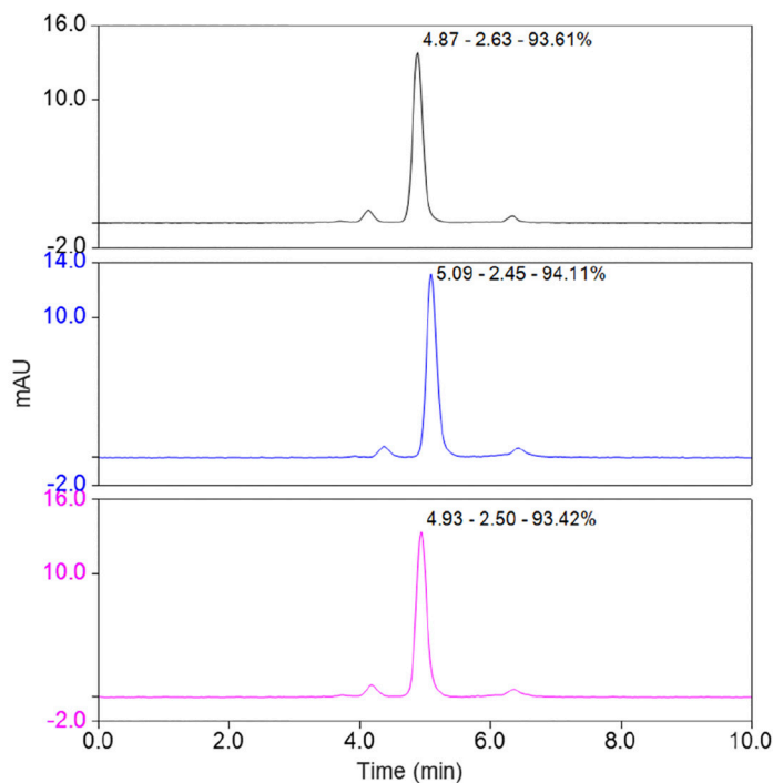
Figure 8. Chromatograms of AAV3 using three different lots of 3 \mu m SurePac Bio 550 SEC MDi columns using UV detection at 280 nm. Peak label: RT (min) - Resolution between monomer and HMWS - %Area
